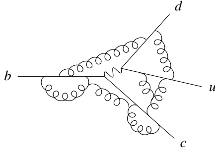
FIG. 1. The nonleptonic decay of a b quark.
